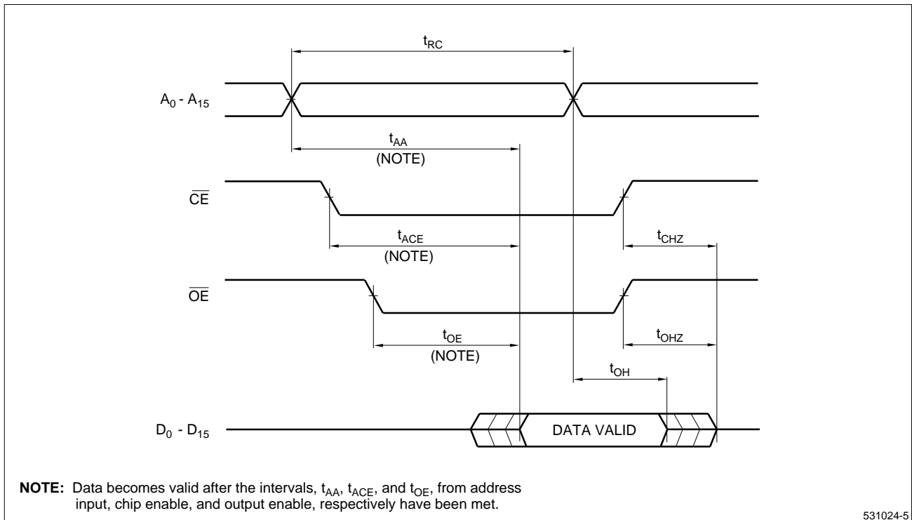
Figure 5. Timing Diagram
