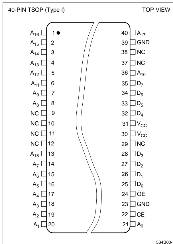
Figure 1. Pin Connections for TSOP Package
