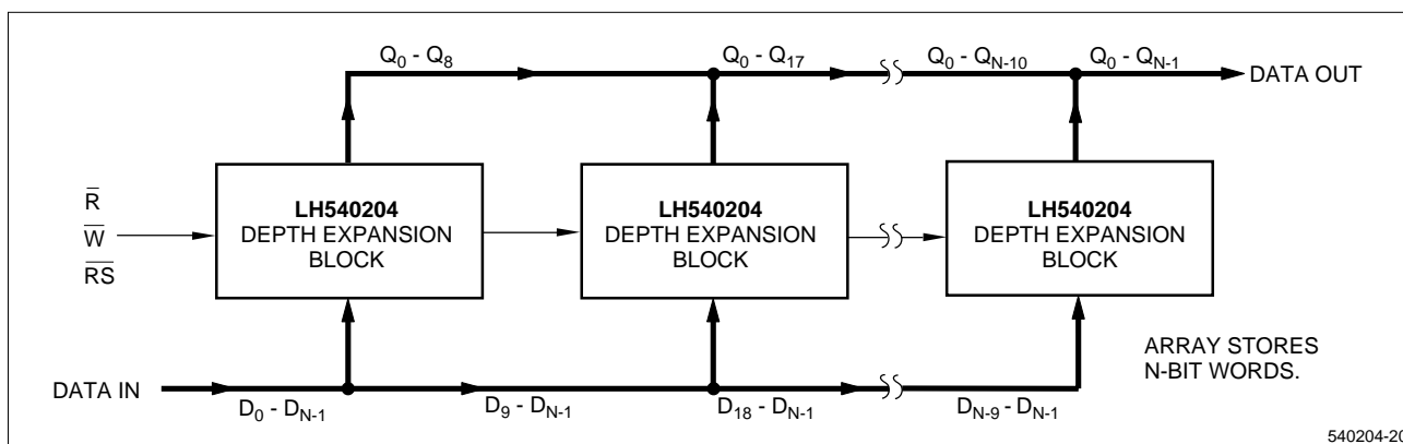
Figure 7. Compound FIFO Expansion
