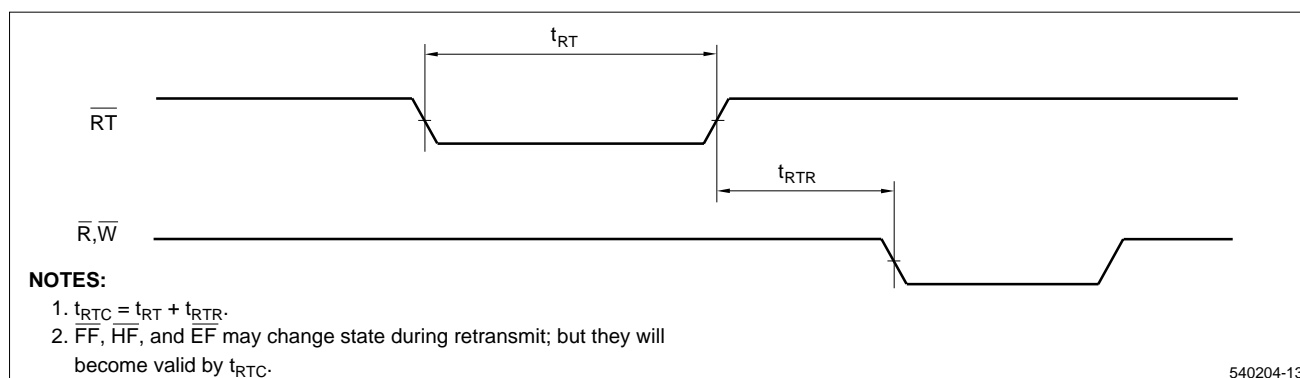
Figure 19. Retransmit Timing
