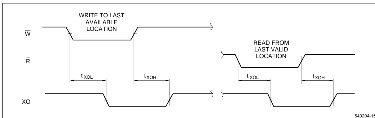
Figure 20. Expansion-Out Timing
