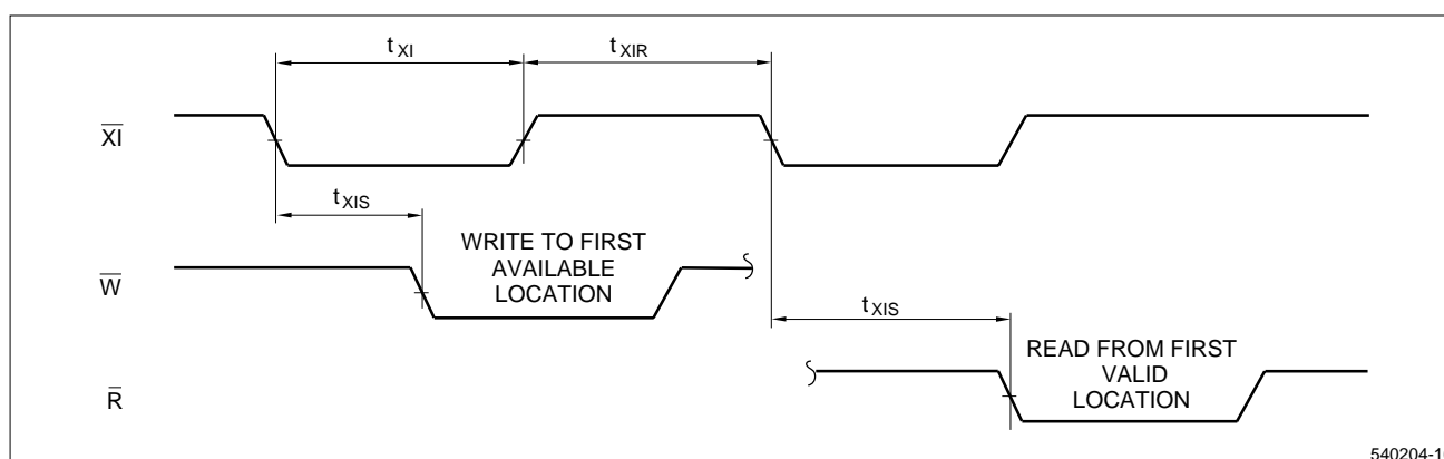
Figure 21. Expansion-In Timing
