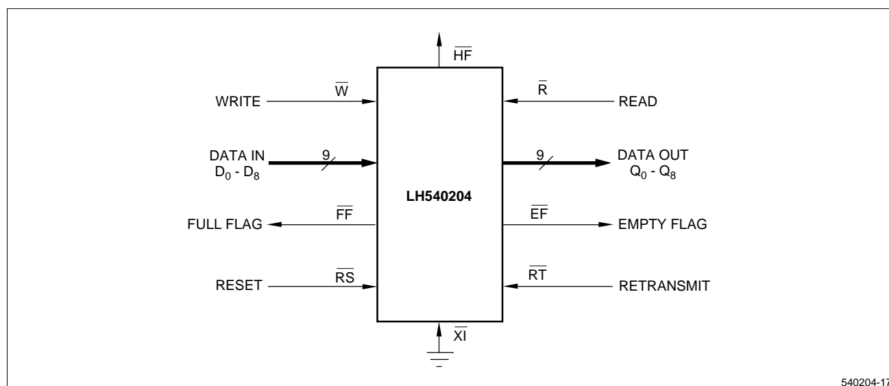
Figure 4. Standalone FIFO (4096 × 9)
