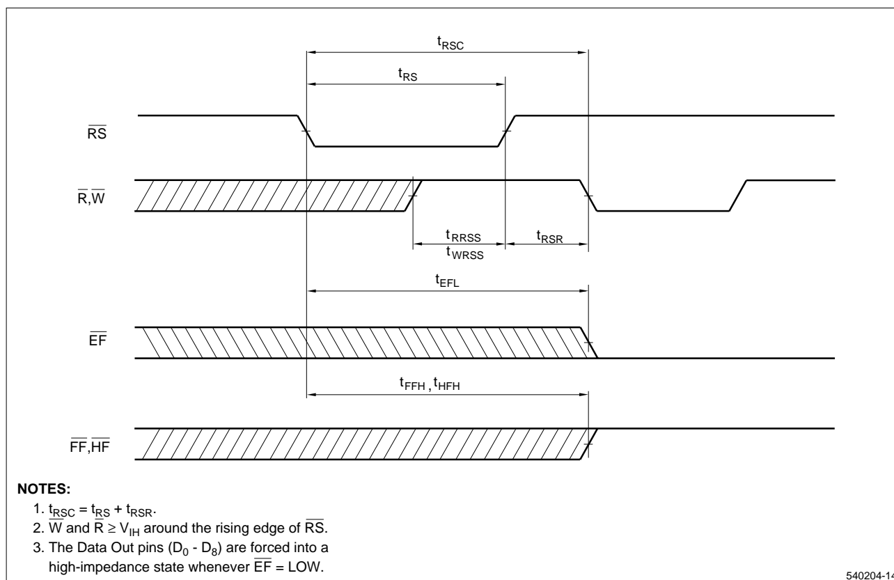
Figure 10. Reset Timing
