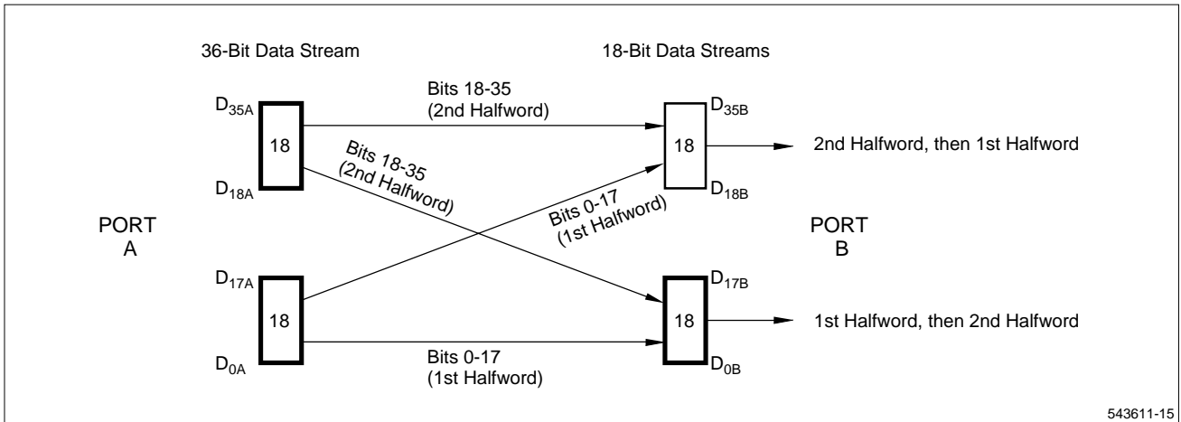
Figure 8a. 36-to-18 Funnelling Through FIFO #1
