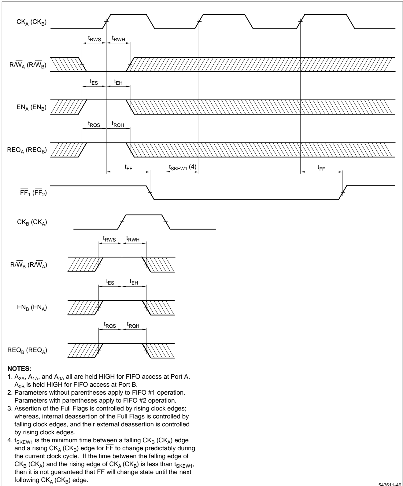
Figure 23. Full Flag Timing, When Synchronous
