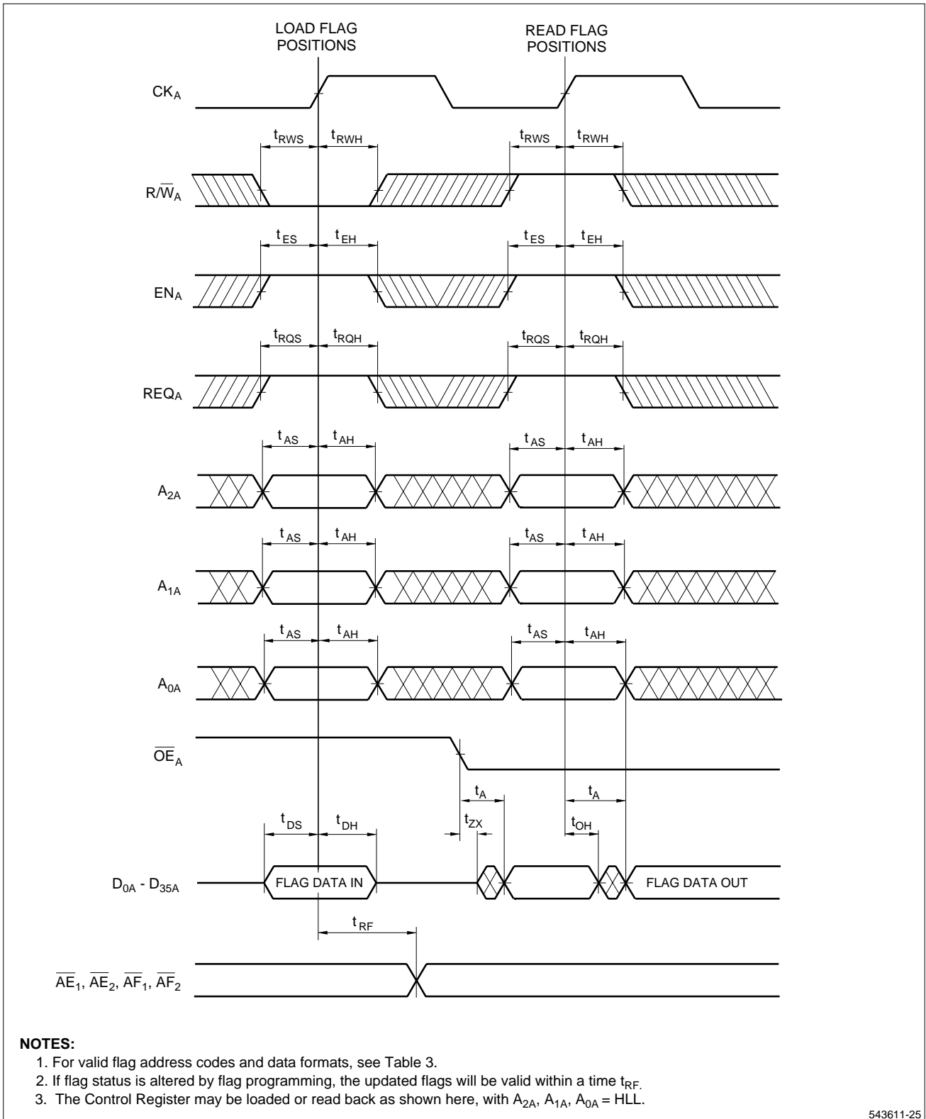
Figure 17. Flag Programming
