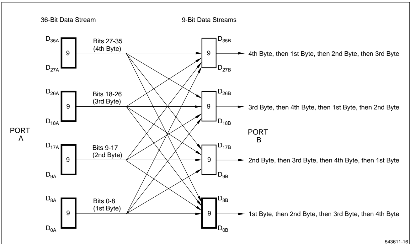
Figure 8b. 36-to-9 Funnelling Through FIFO #1
