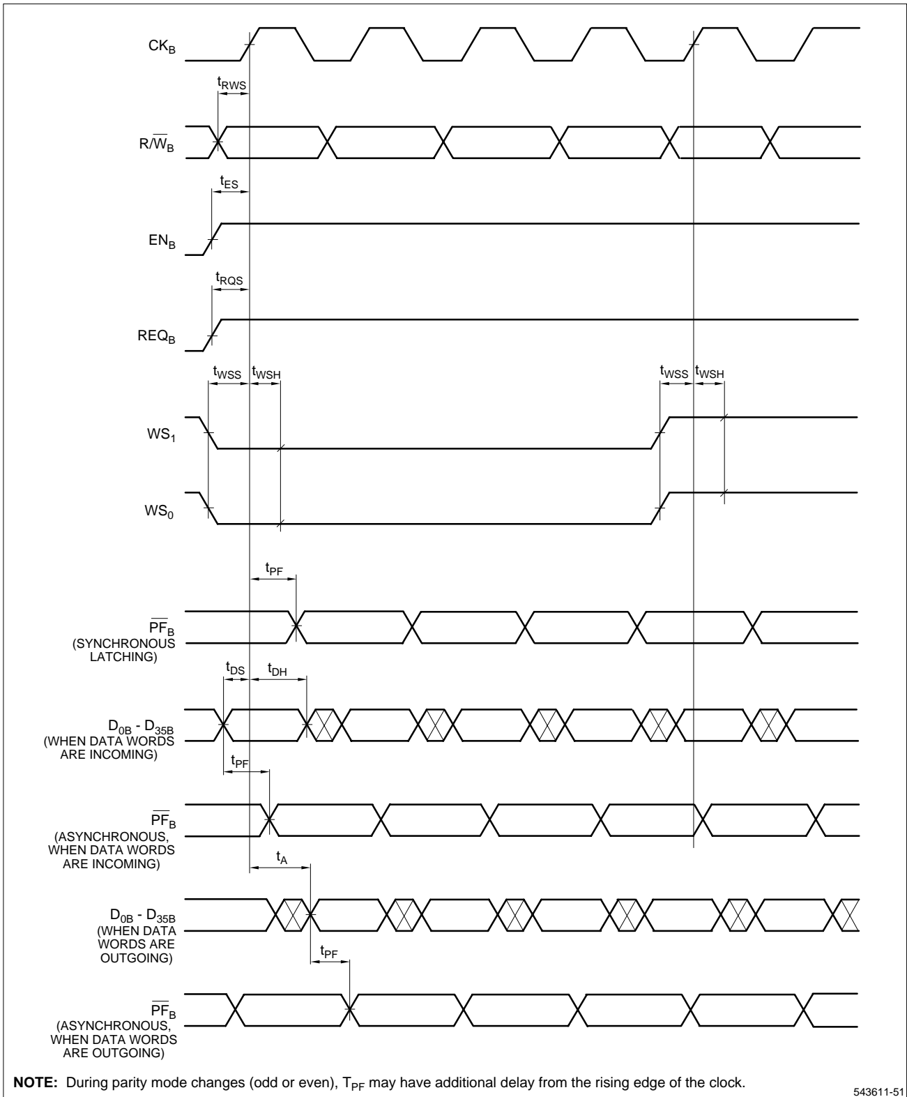
Figure 42. Parity Generation
