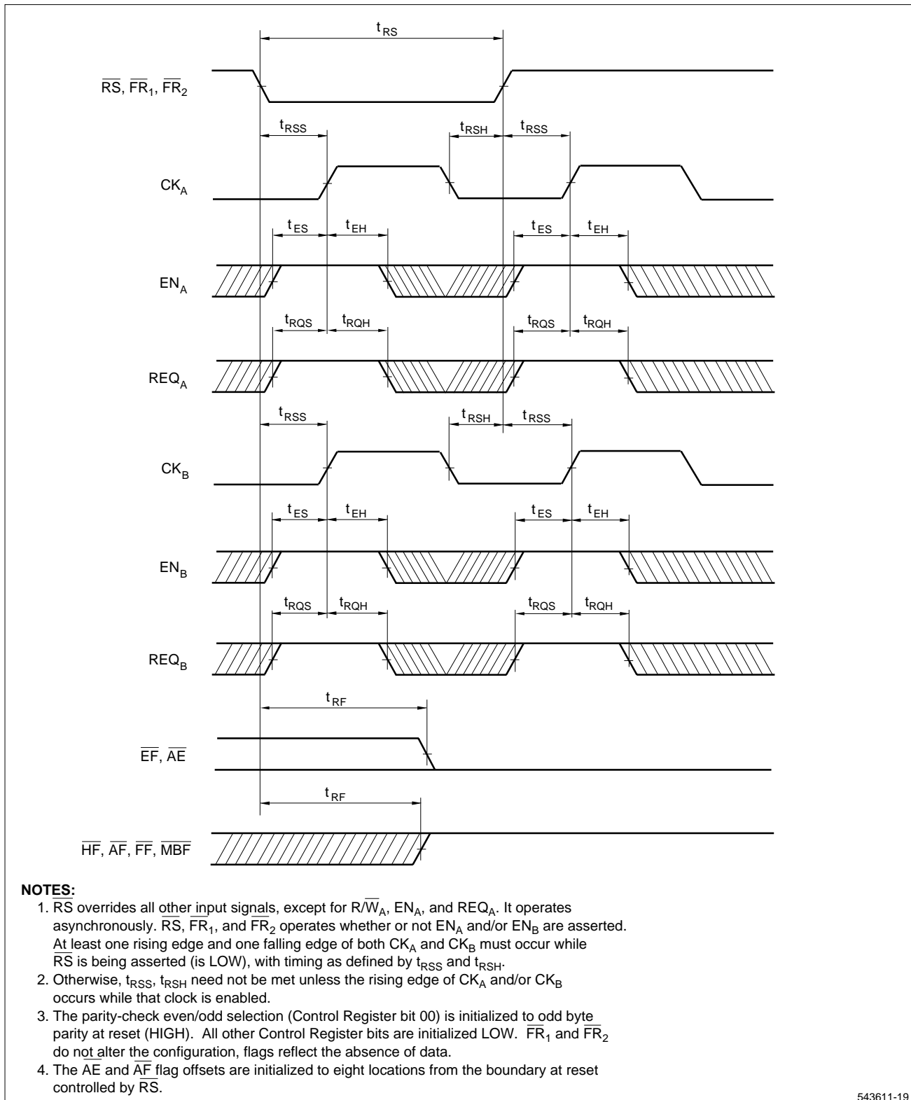
Figure 11. Reset Timing
