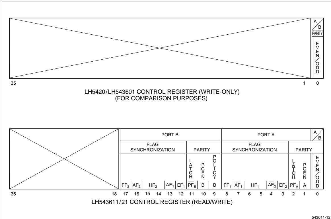
Figure 10. LH5420/LH543601 and LH543611/21 Control-Register Formats
