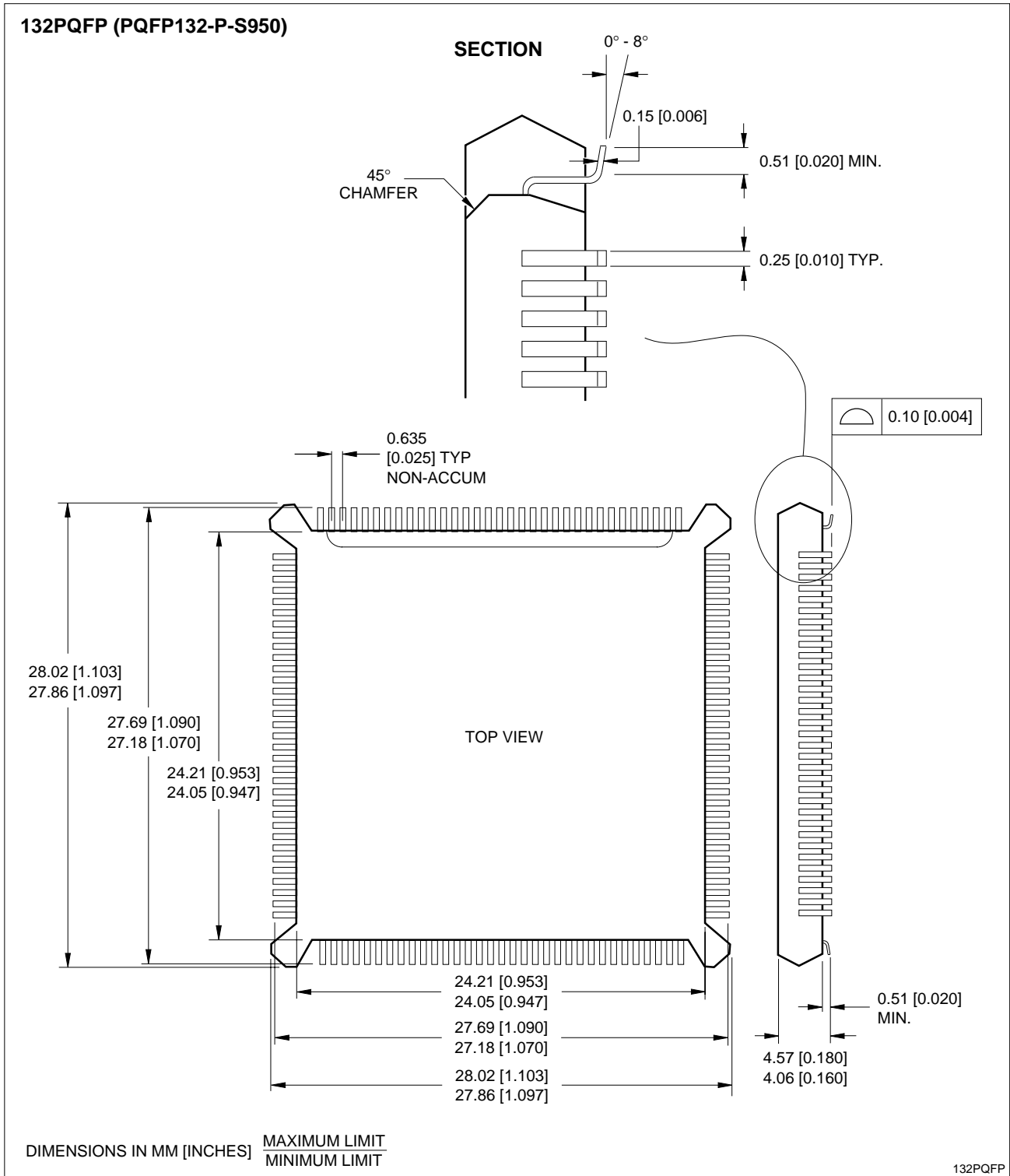
132-pin PQFP
