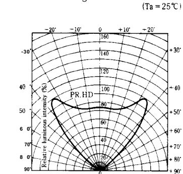
Radiation Diagram
