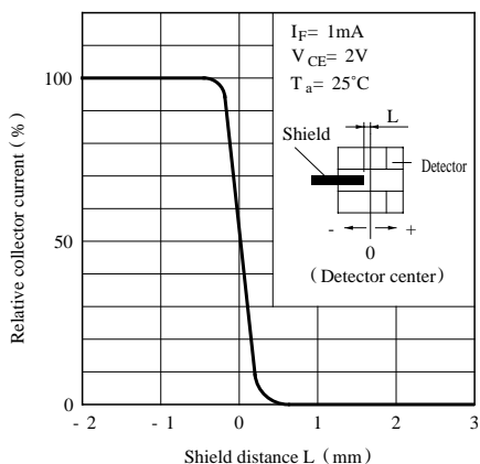
Fig.10-b Relative Collector Current vs. Shield Distance (1) (GP1L22)
