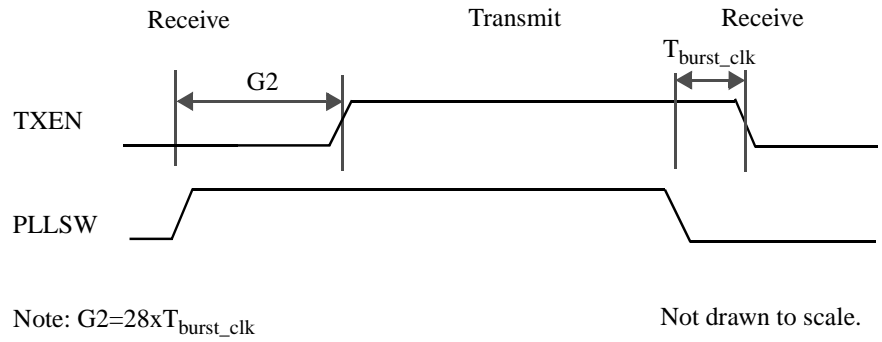
Figure 13. PLLSW Timing (Full-Duplex Mode)
