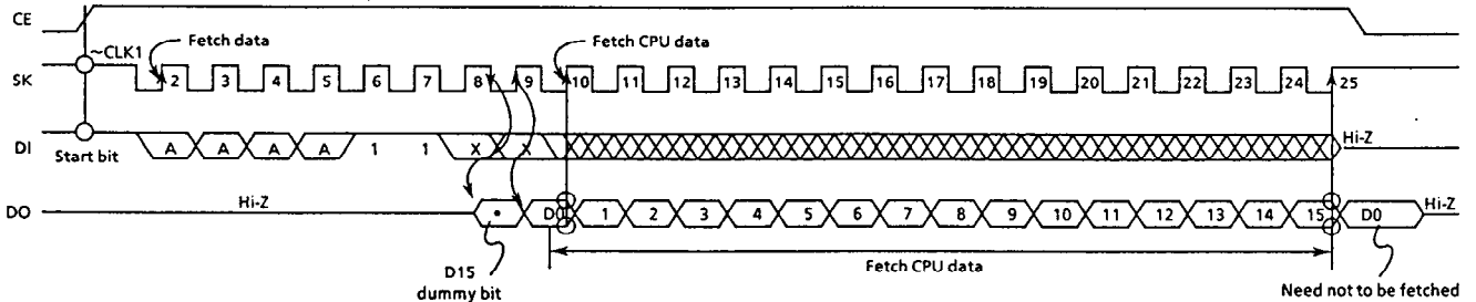
Figure 13 Read mode timing(S-24H45, S-24S45)
