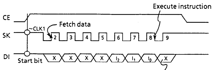
Figure 17 Other operation mode timing
