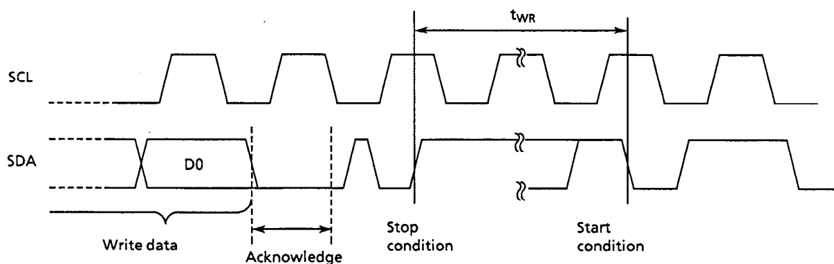
Figure 5 Write Cycle
