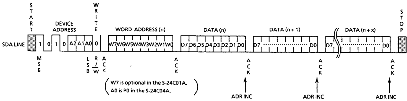
Figure 11 Page Write
