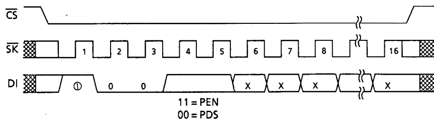
Figure 7 PEN/PDS Timing
