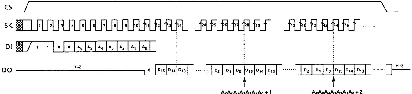
Figure 5 Read Timing (S-29L220A)
