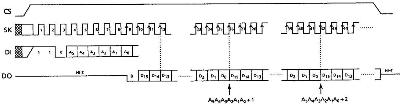
Figure 4 Read Timing (S-29L130A)
