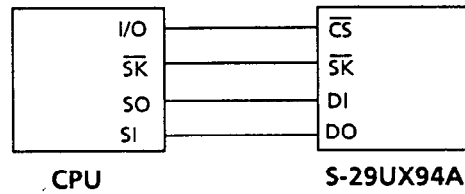
Figure 9 Connectin Example
