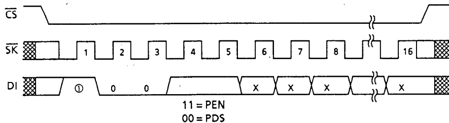
Figure 7 PEN/PDS Timing
