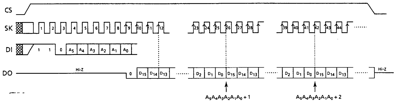
Figure 4 Read Timing (S-29U131A)
