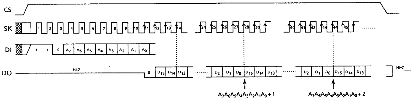
Figure 6 Read Timing (S-29U331A)
