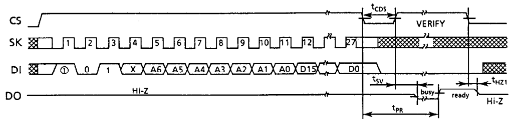
Figure 8 WRITE Timing (S-29U221A)
