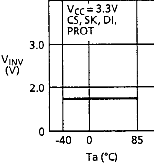
1.25 Input inversion voltage V_{INV} – Ambient temperature T_a
