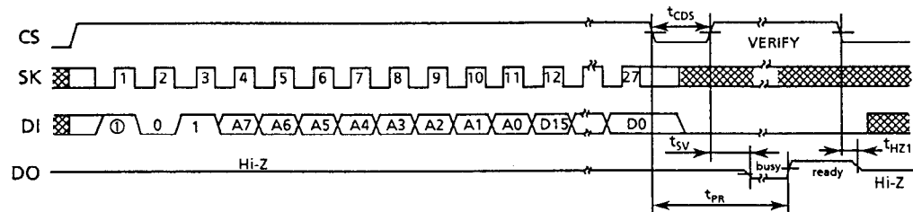
Figure 9 WRITE Timing (S-29U331A)
