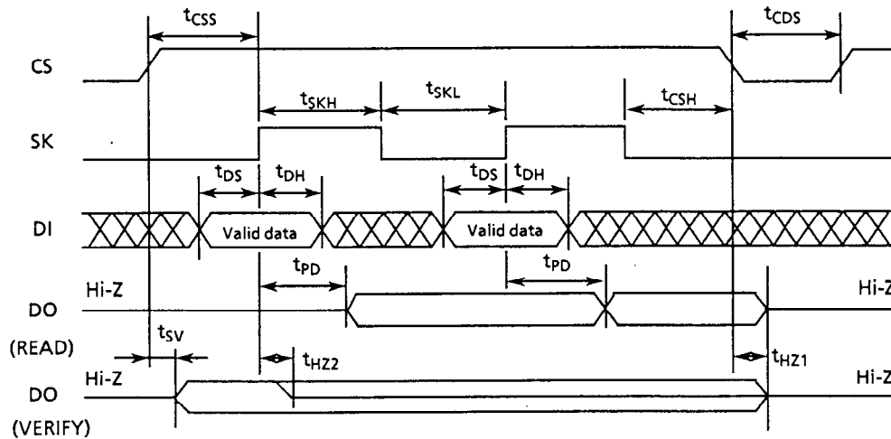
Figure 3 Timing Chart
