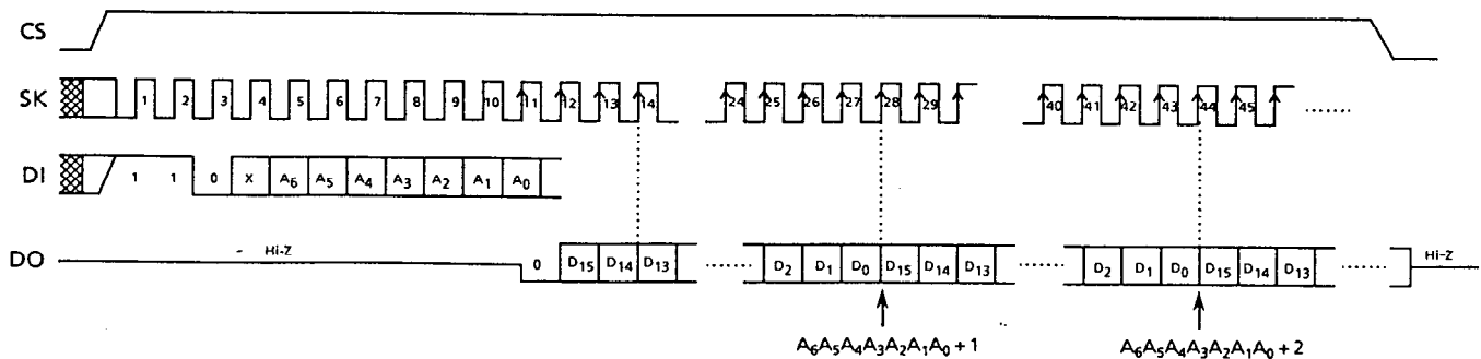
Figure 5 Read Timing (S-29U221A)
