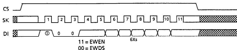
Figure 14 EWEN/EWDS Timing (S-29U221A)
