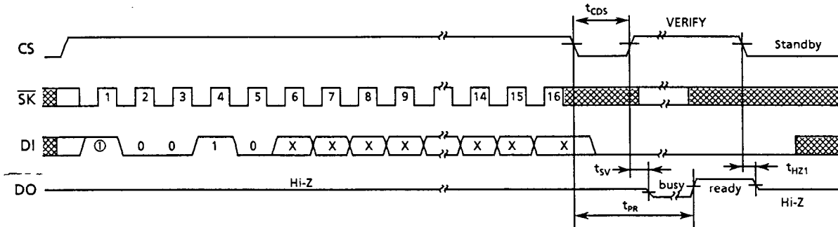
Figure 8 ERAL Timing
