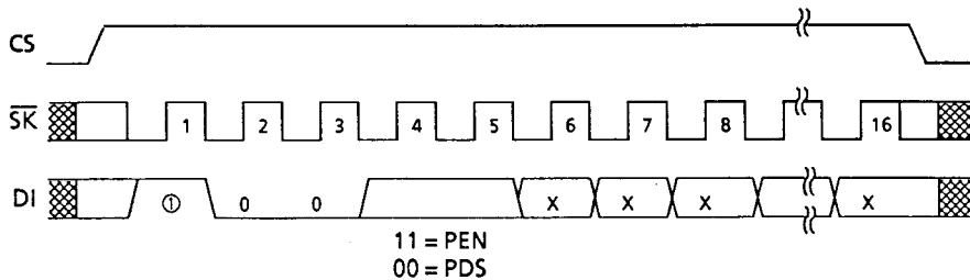
Figure 9 PEN/PDS Timing
