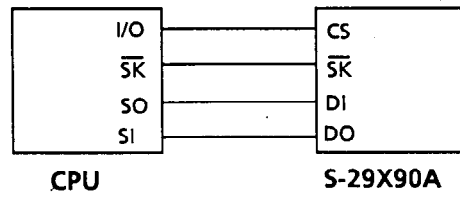
Figure 11 Connectin Example
