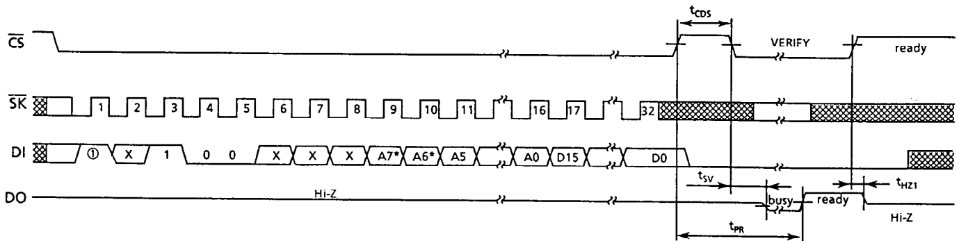
Figure 6 WRITE Timing (S-29394A)
