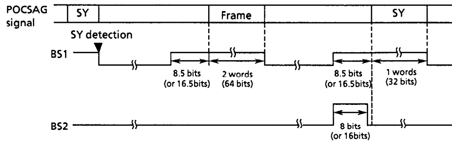
Figure 19 Battery saving
