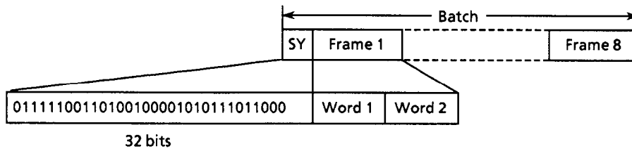
Figure 7 Batch configuration
