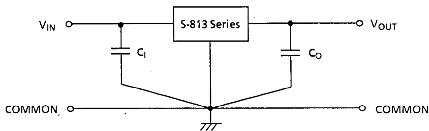
Figure 20 Standard circuit
