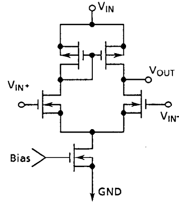
Figure 6 Error amplifier
