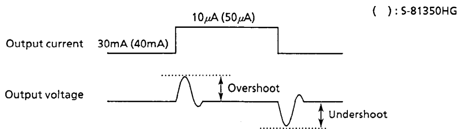
Figure 12 Ringing waveform
