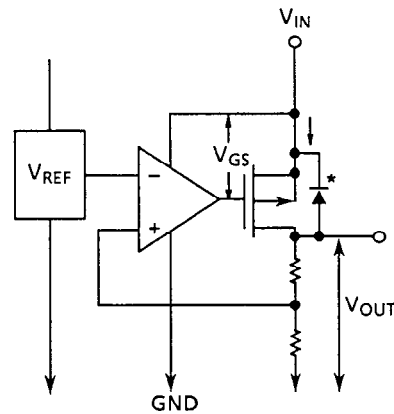
Figure 7 Control transistor
