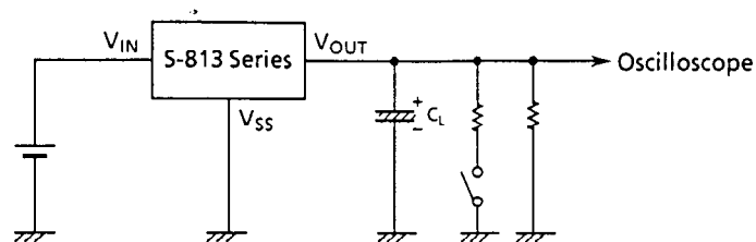
Figure 13 Measuring circuit
