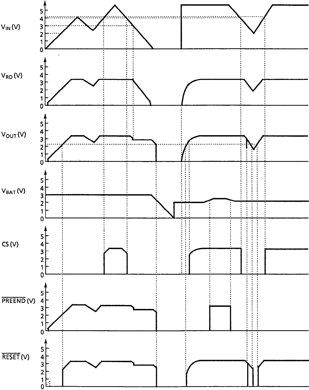
CS, and \overline{PREEND} and \overline{RESET} are pulled up to V_{OUT} .
