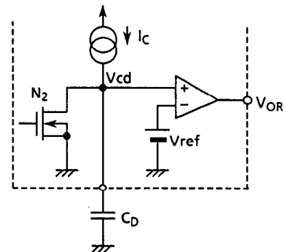
Figure 9 Delay circuit
