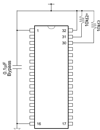
Figure 3: System Power Mode
