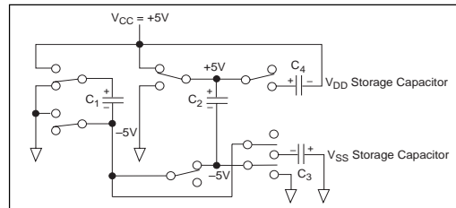
Figure 13a. Charge Pump Phase 1 for \pm 10\text{V} .
