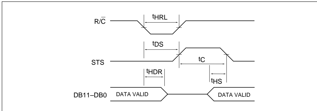
Figure 8. Low Pulse for R/\overline{C} — Outputs Enabled After Conversion
