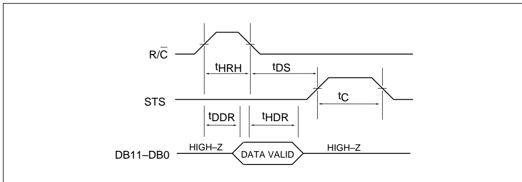
Figure 9. High Pulse For R/\overline{C} — Outputs Enabled While R/\overline{C} is High, Otherwise High Impedance
