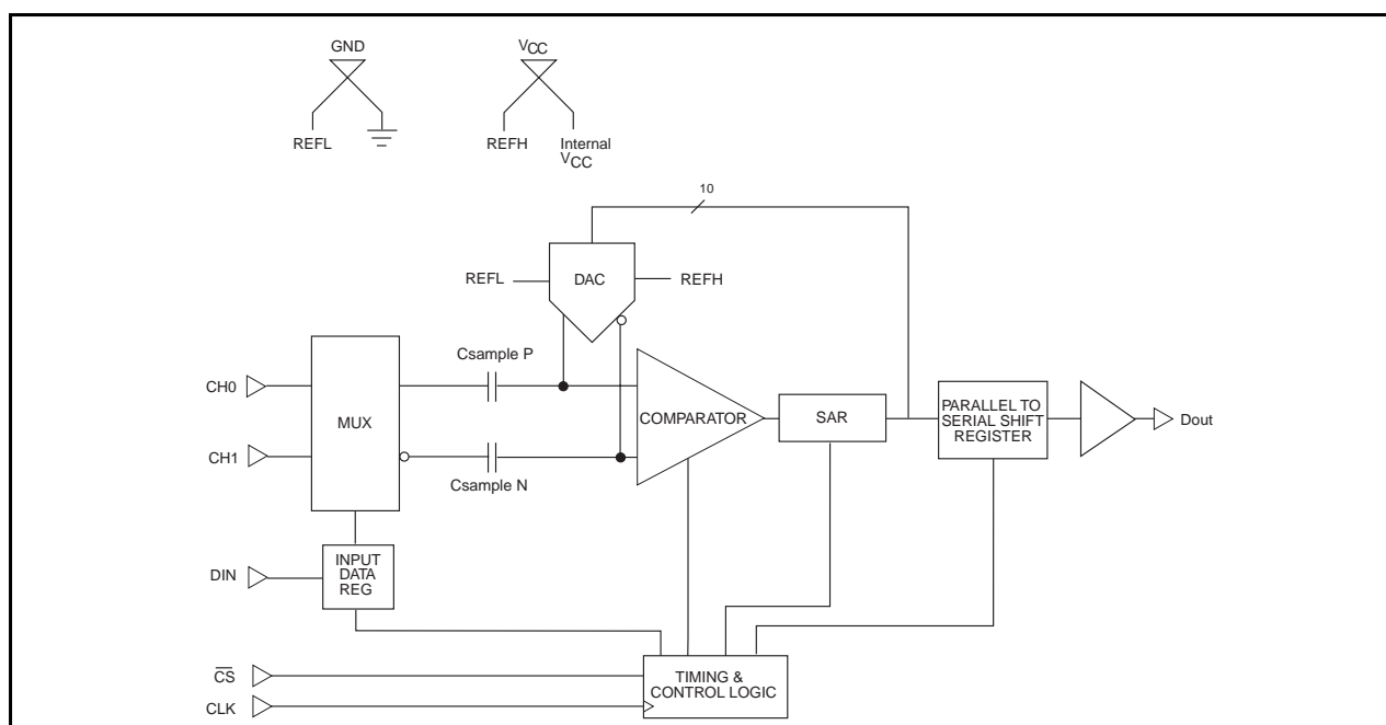
SP8537 Block Diagram
