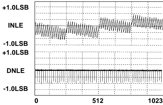
Vcc = 5.00V
