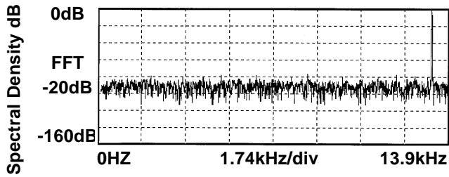
FFT 20 dB/div Vcc =5V
