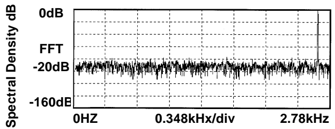
FFT 20 dB/div Vcc =3V
