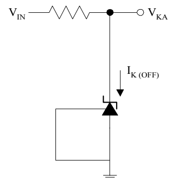
Figure 1c. Test Circuit 3
