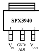
SOT-223 Package
