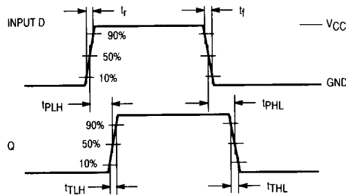
Figure 1. Switching Waveforms
