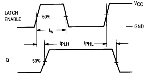
Figure 2. Switching Waveforms
