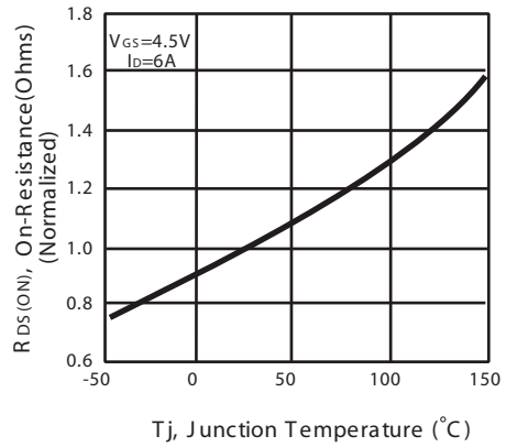
Figure 4. On-R resistance Variation with Temperature
