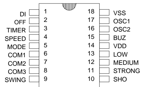
SM3502-B 18PIN
