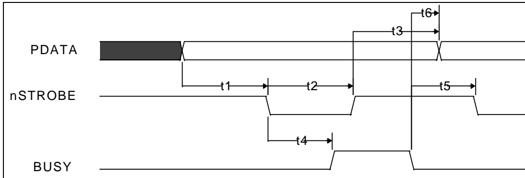
FIGURE 29 - PARALLEL PORT FIFO TIMING
