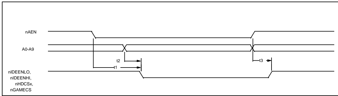
FIGURE 23 - IDE INTERFACE TIMING
