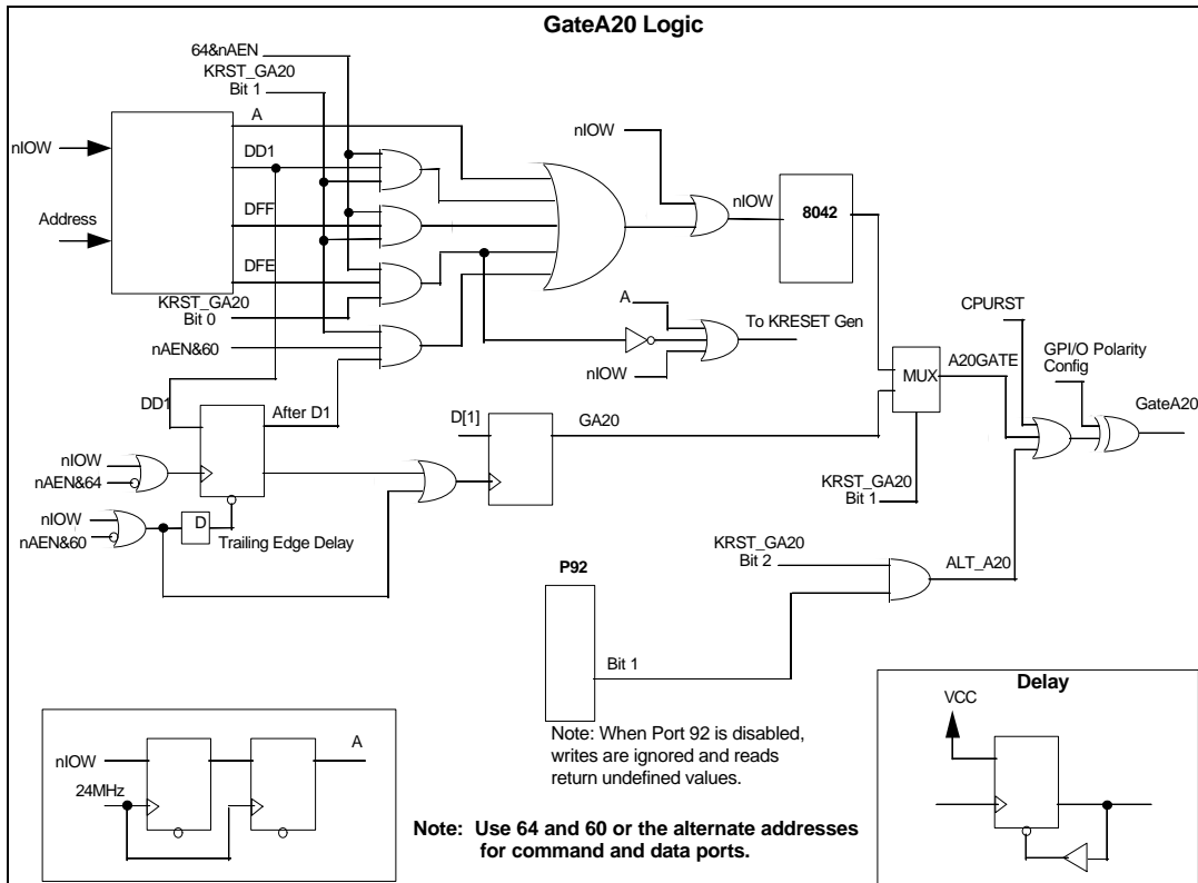
FIGURE 7 - GATEA20 GENERATION LOGIC
