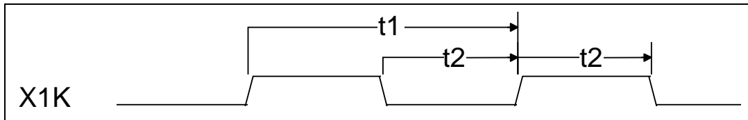
FIGURE 16A - INPUT CLOCK TIMING
