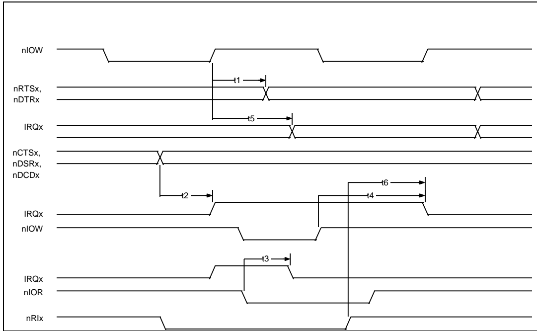
FIGURE 22 - SERIAL PORT TIMING
