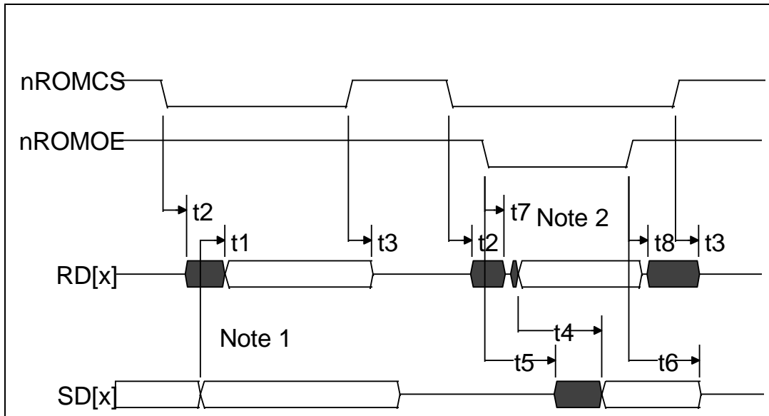
FIGURE 19 - ROM INTERFACE TIMING
