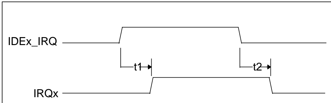
FIGURE 17 - IRQ TIMING
