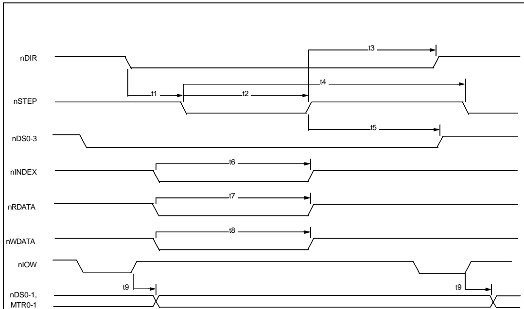
FIGURE 21 - DISK DRIVE TIMING (AT MODE ONLY)
