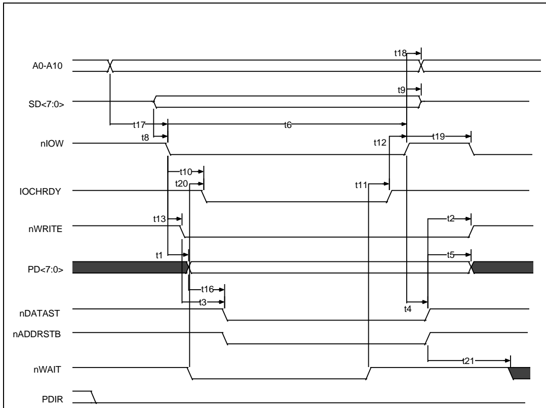
FIGURE 27A - EPP 1.7 DATA OR ADDRESS WRITE CYCLE
