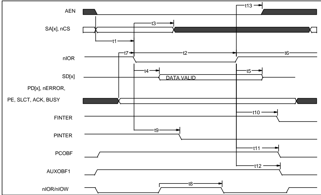
FIGURE 14 - ISA READ
