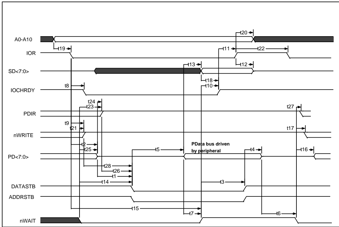
FIGURE 26A - EPP 1.9 DATA OR ADDRESS READ CYCLE
