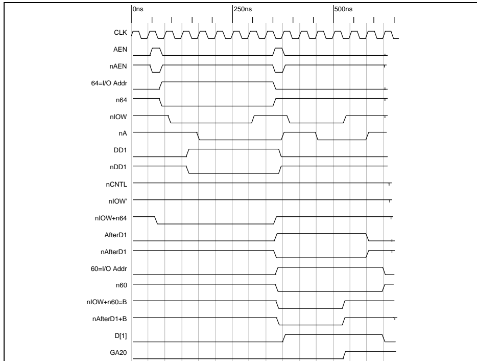
FIGURE 8 - GATE A20 TURN-ON SEQUENCE TIMING
