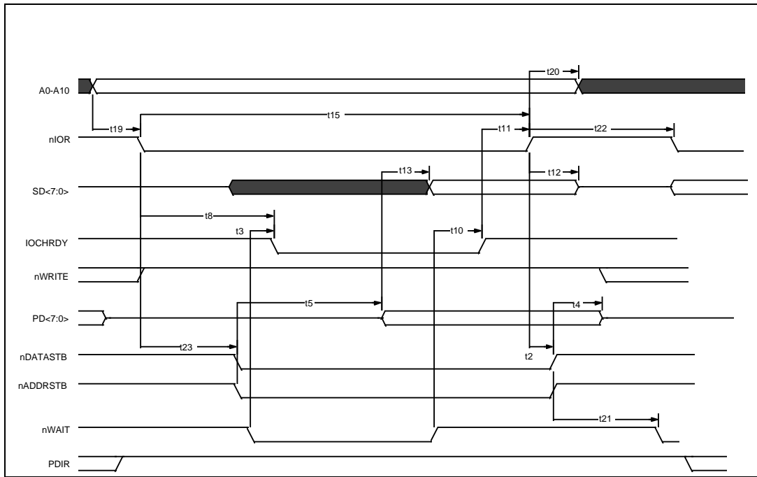
FIGURE 28A - EPP 1.7 DATA OR ADDRESS READ CYCLE
