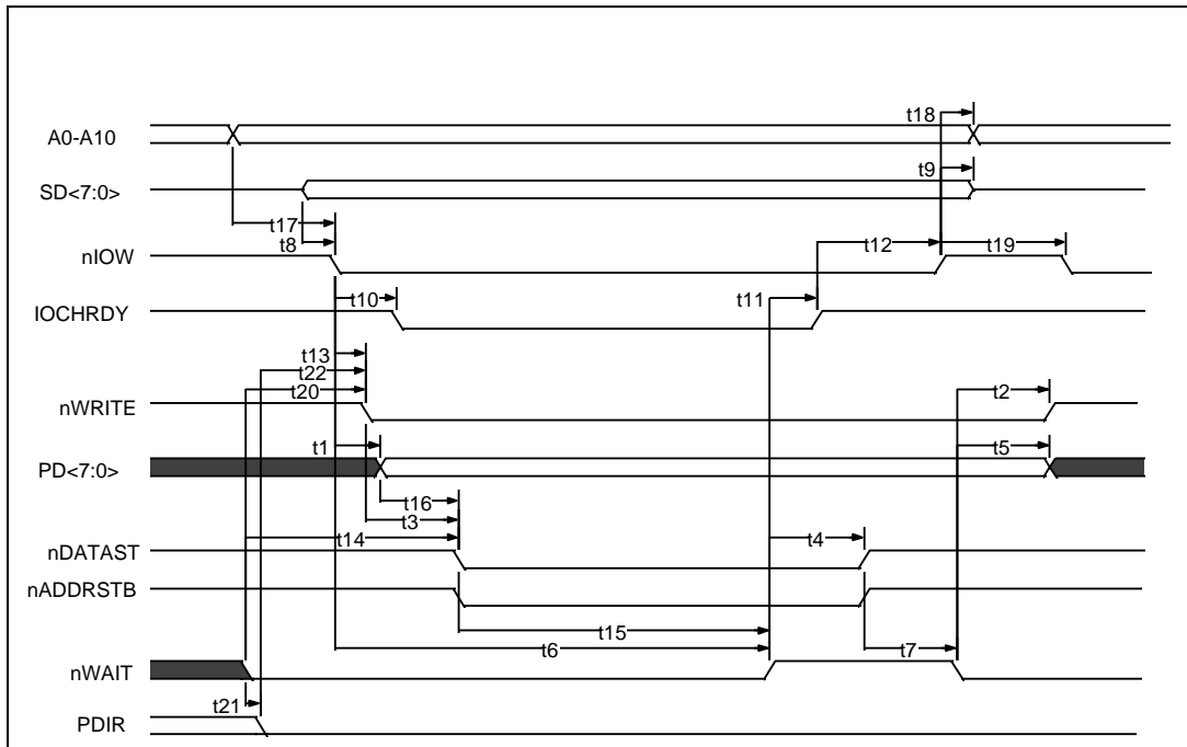
FIGURE 25A - EPP 1.9 DATA OR ADDRESS WRITE CYCLE
