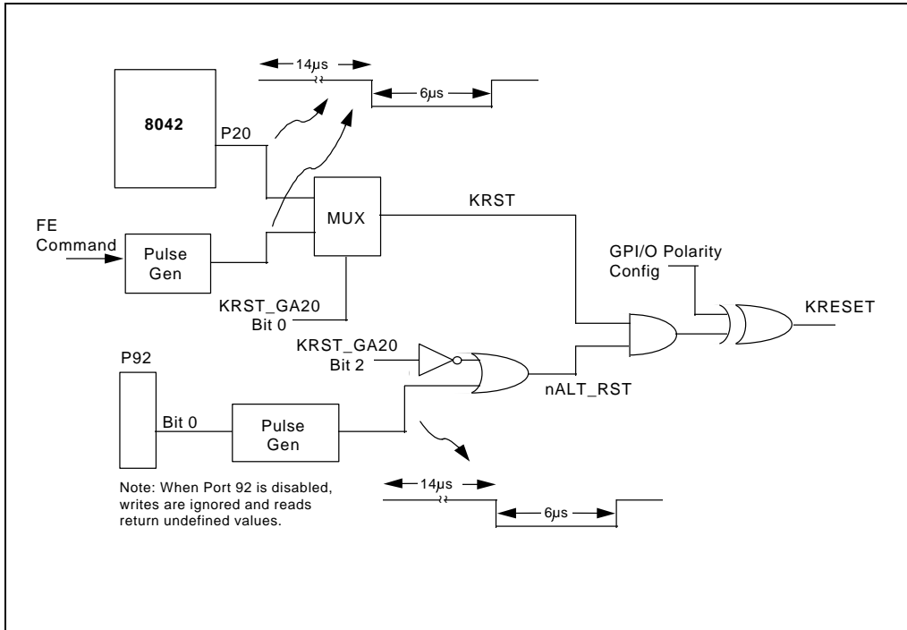
FIGURE 6 - KRESET GENERATION
