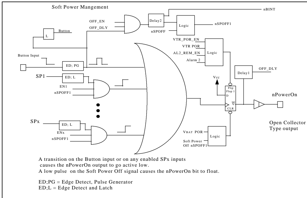
FIGURE 9 - SOFT POWER MANAGEMENT FUNCTIONAL DIAGRAM
