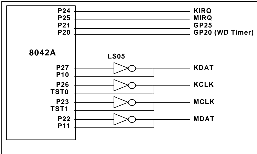
FIGURE 5 - KEYBOARD AND MOUSE CONTROLLER
