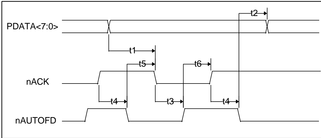
FIGURE 31 - ECP PARALLEL PORT REVERSE TIMING
