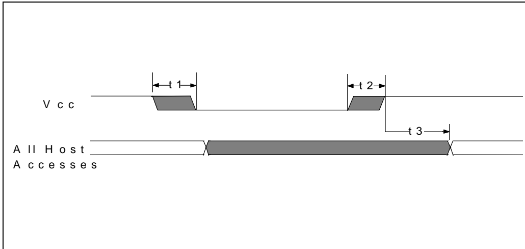
FIGURE 12 - POWER-UP TIMING
