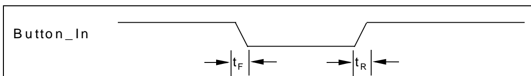
FIGURE 10 - BUTTON INPUT TIMING
