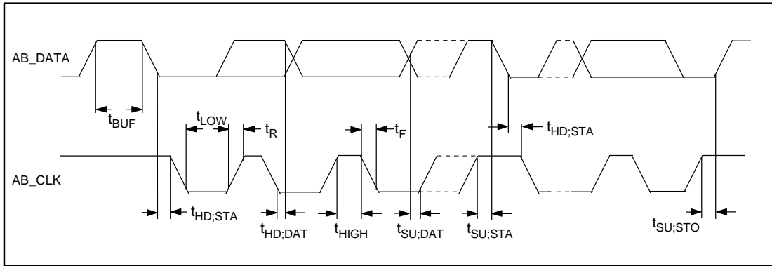
FIGURE 32 - ACCESS.BUS TIMING
