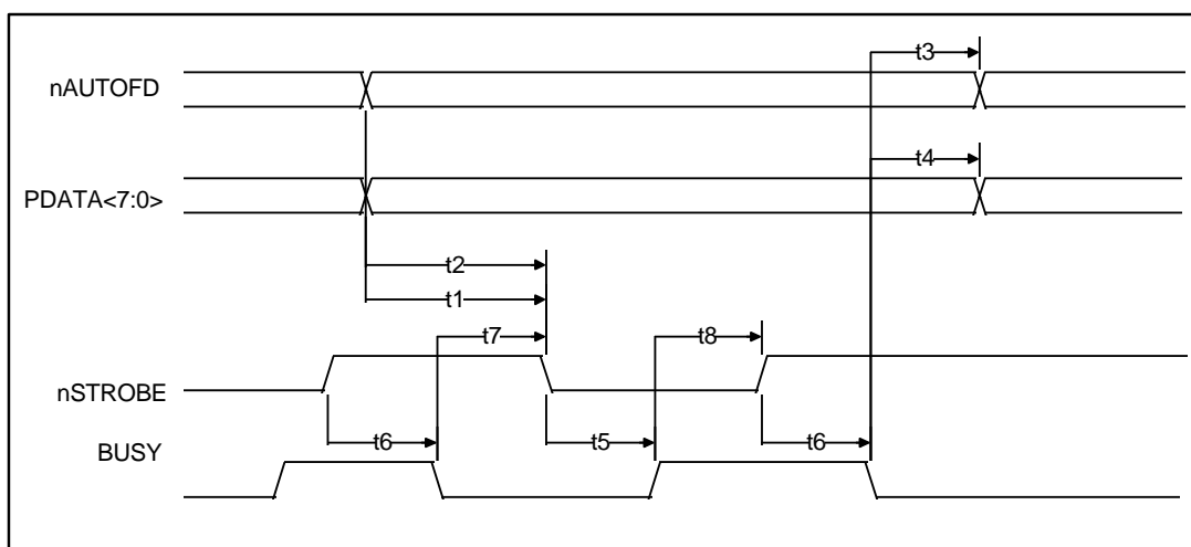
FIGURE 30 - ECP PARALLEL PORT FORWARD TIMING
