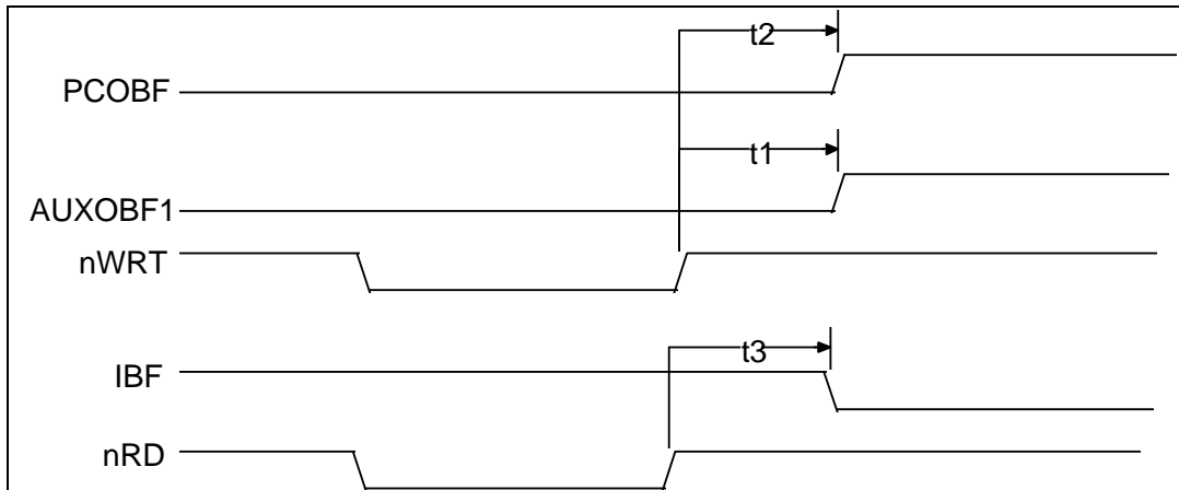
FIGURE 15 - INTERNAL 8042 CPU TIMING
