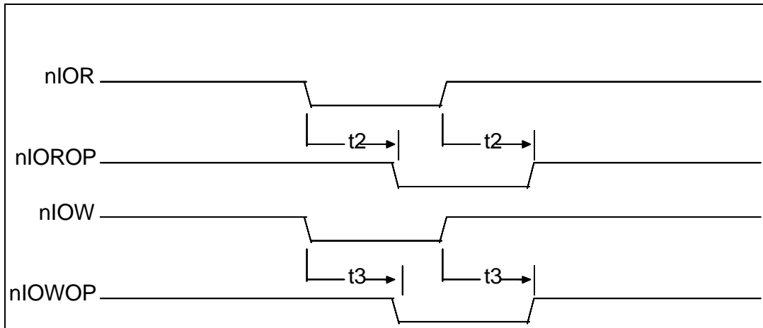
FIGURE 18 - nIOROP, nIOWOP TIMING
