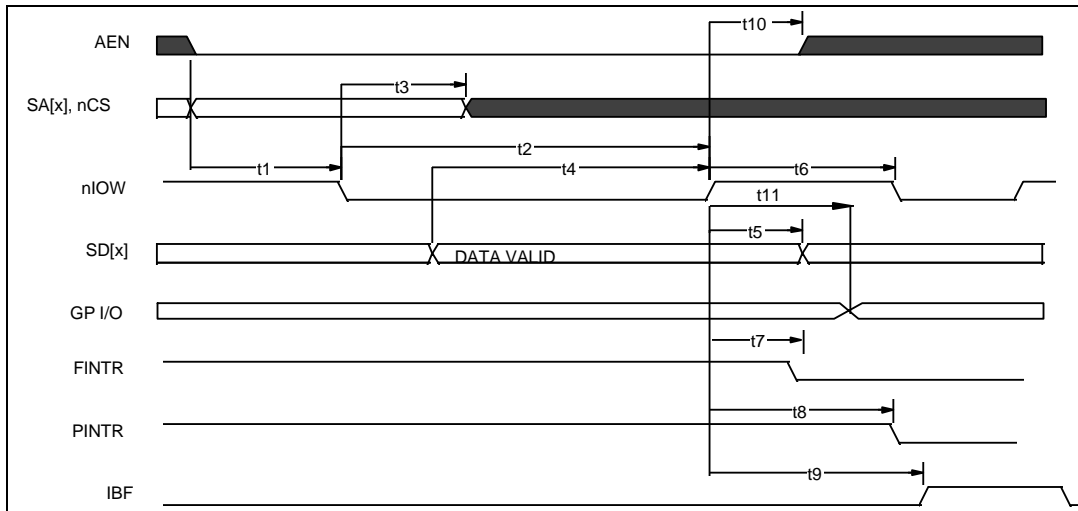
FIGURE 13 - ISA WRITE
