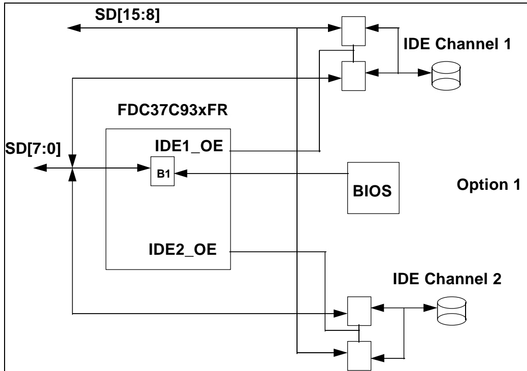
FIGURE 3 - BIOS BUFFER
