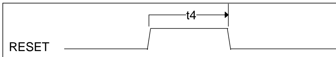
FIGURE 16B - RESET TIMING
