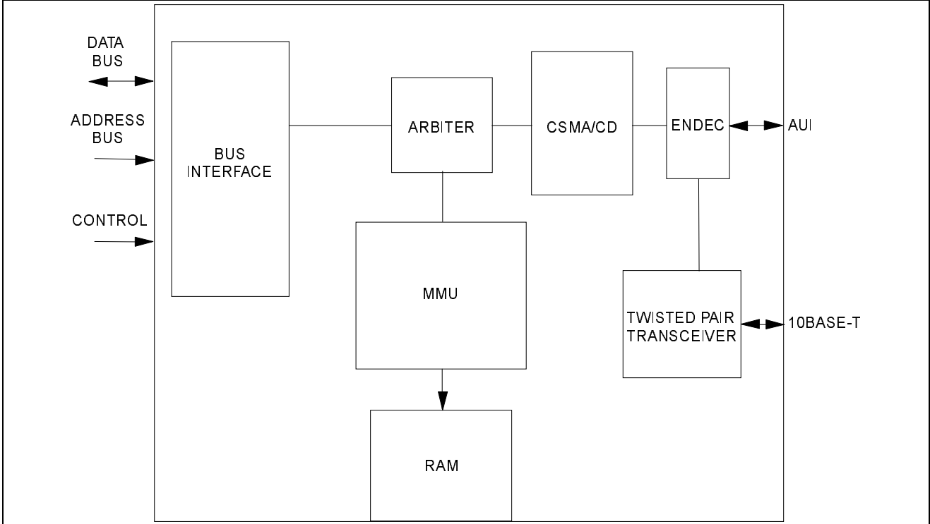
FIGURE 2 - SMC91C94 INTERNAL BLOCK DIAGRAM
