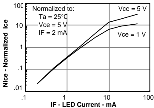
Figure 4. Normalized non-saturated and saturated Nice versus LED current
