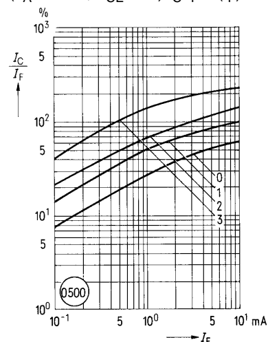
Figure 4. Current transfer ratio versus diode current ( T_A=0\text{ °C} , V_{CE}=5\text{ V} ) I_C/I_F=f(I_F)
