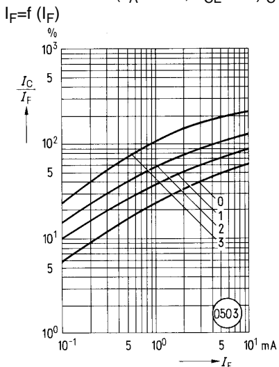
Figure 5. Current transfer ratio versus diode current ( T_A=25\text{ °C} , V_{CE}=5\text{ V} ) I_C/I_F=f(I_F)
