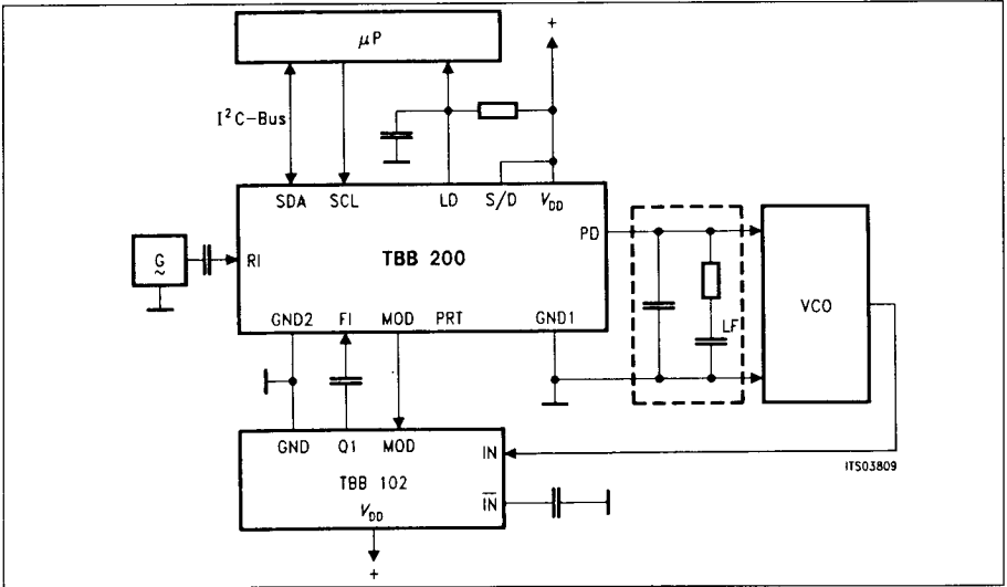
Operation: dual-modulus ( f_{max} = 30 MHz at FI)
