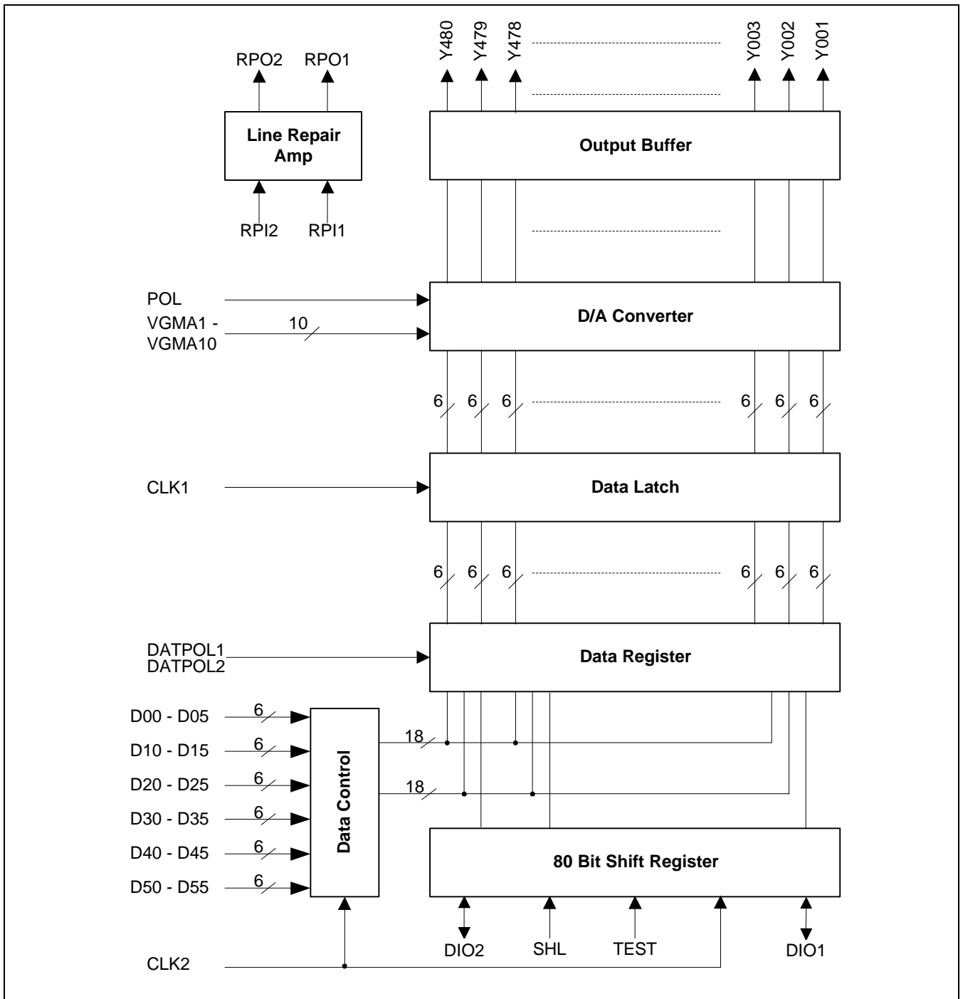
Figure 1. S6C0676 Block Diagram
