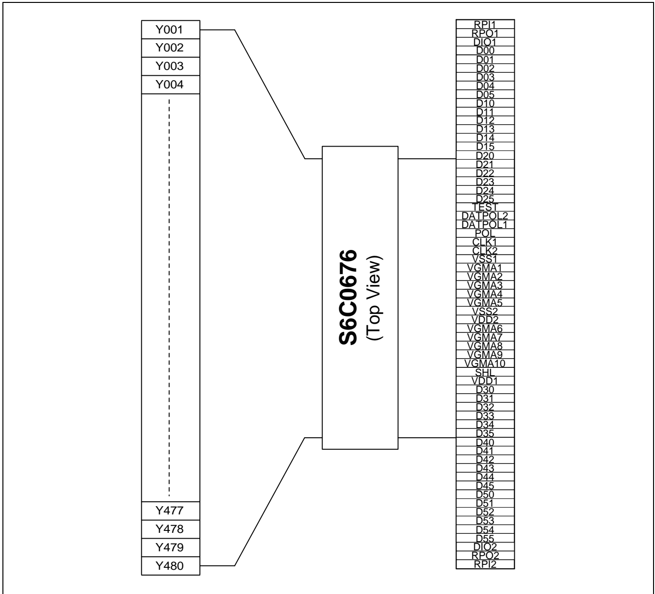
Figure 2. S6C0676 Pin Assignments
