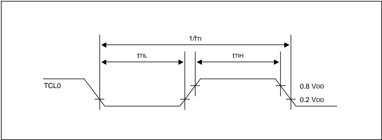
Figure 14-7. TCL Timing
