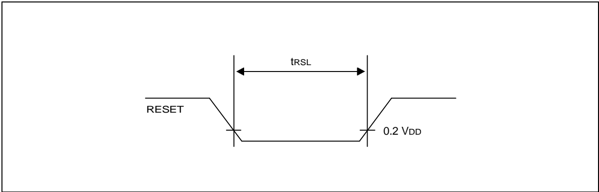
Figure 14-8. Input Timing for RESET Signal
