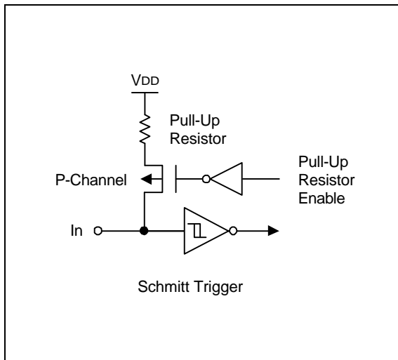
Figure 1-4. Pin Circuit Type A-3
