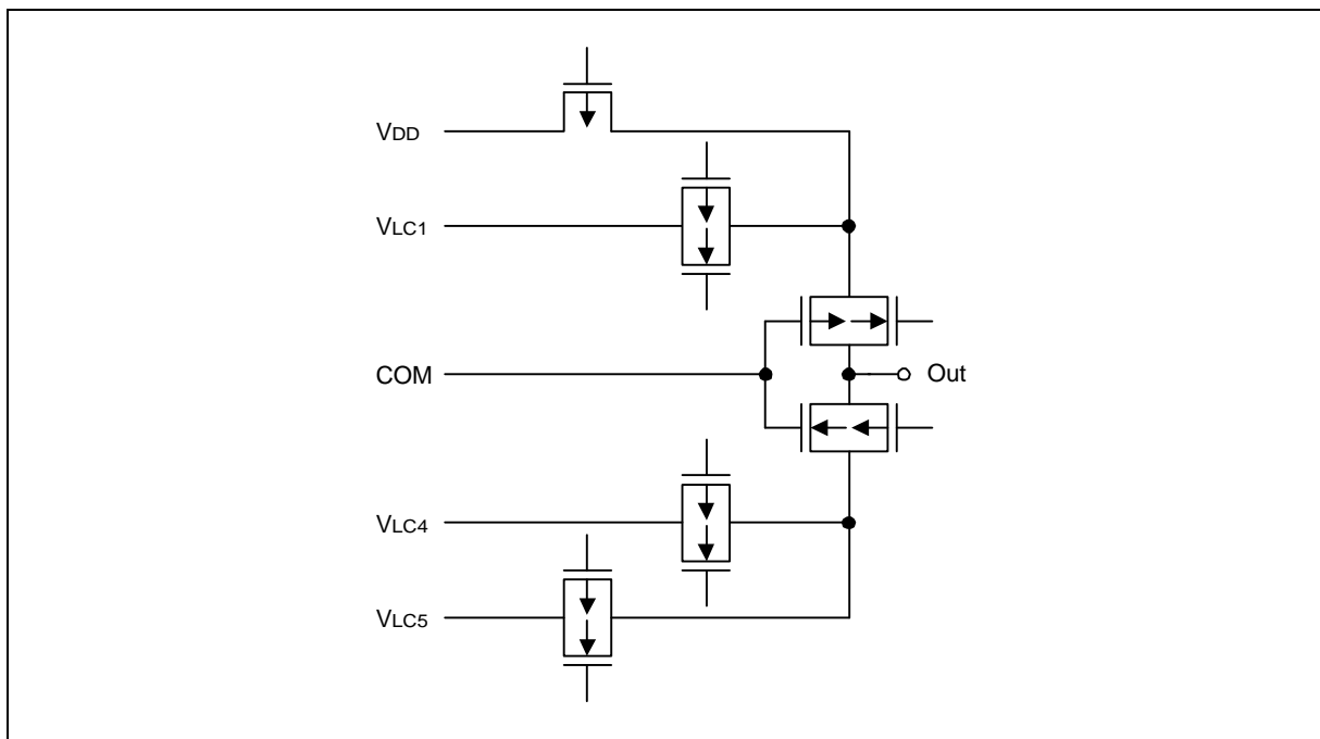
Figure 1-10. Pin Circuit Type H-3
