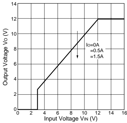
Rise Characteristics(SI-3120N)
