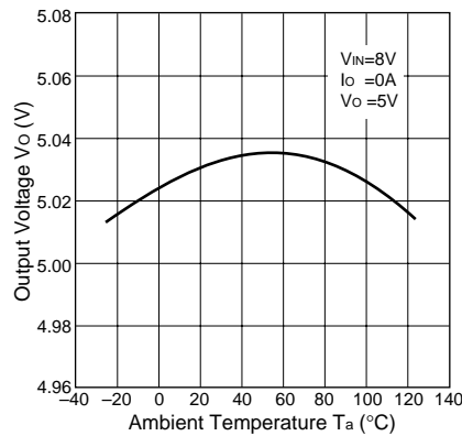
Temperature Coefficient of Output Voltage(SI-3051N)
