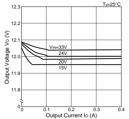
Load Regulation(SI-8402L)
