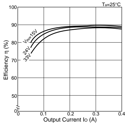
Efficiency Characteristics(SI-8402L)
