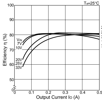
Efficiency Characteristics(SI-8401L)
