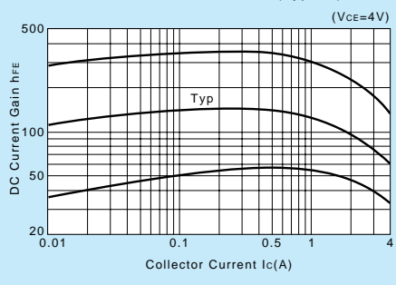
h FE -I c Characteristics (Typical)
