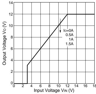
Rise Characteristics(SI-3121N)
