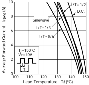
T l —I F (AV) Derating
