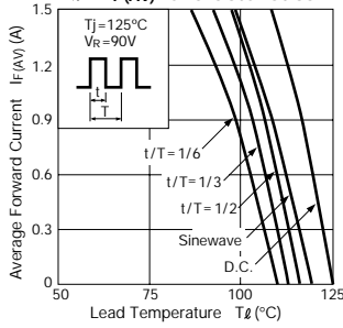
Tl—If(AV) Characteristics
