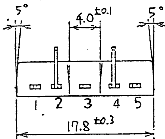
Pin Connection
