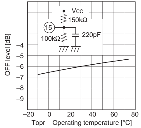
Dropout detection OFF level vs. Operating temperature
