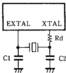
Fig. 10 Recommended oscillation circuit
