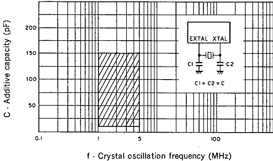
Fig. 9 Crystal oscillation circuit additive capacity calculation chart (Ta = -20 to +75°C, V DD = 4.5 to 5.5 V)
