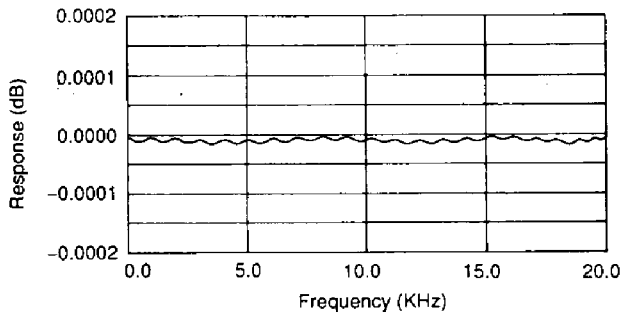
Ripple characteristics
