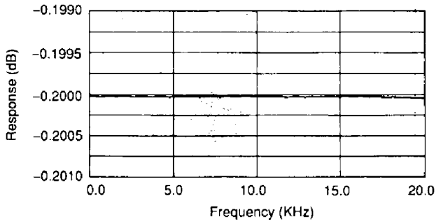
Frequency characteristics
