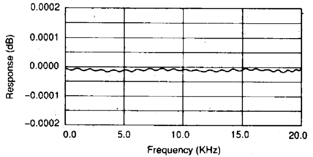
Ripple characteristics
