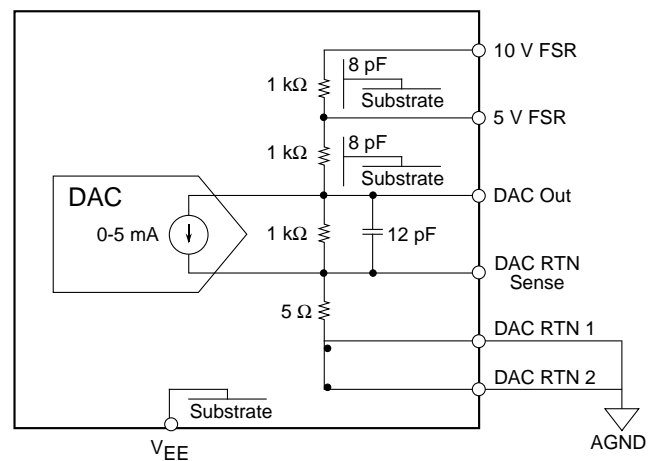
Figure 1 - Equivalent SPT5216 Output Circuit
