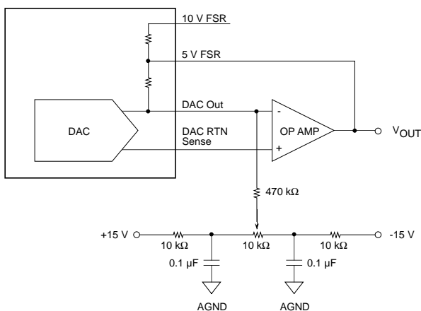
Figure 4 - Offset Compensation
