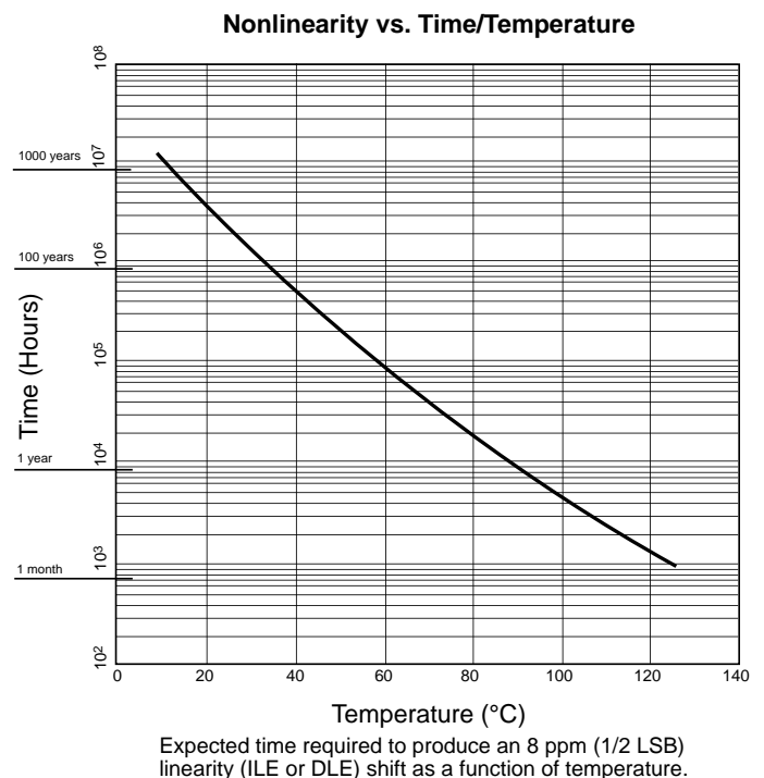
Figure 7 - Linearity Performance over Time
