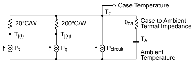
Figure 10: Thermal Model
