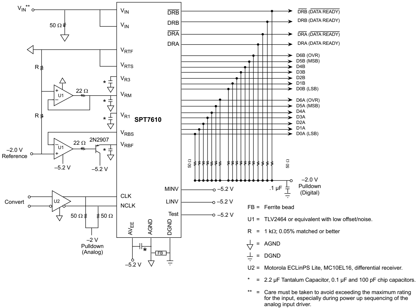
Figure 3 – Typical Interface Circuit
