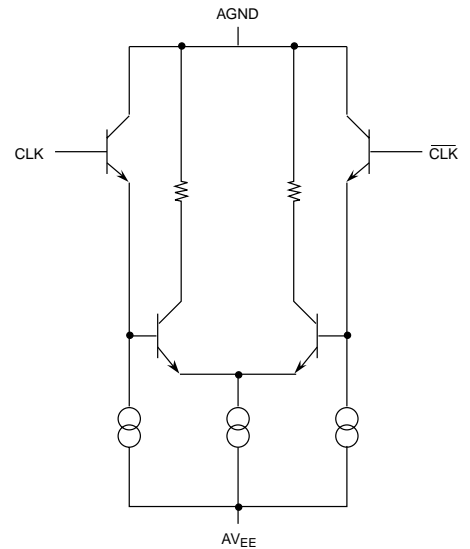
Figure 3C – Clock Input
