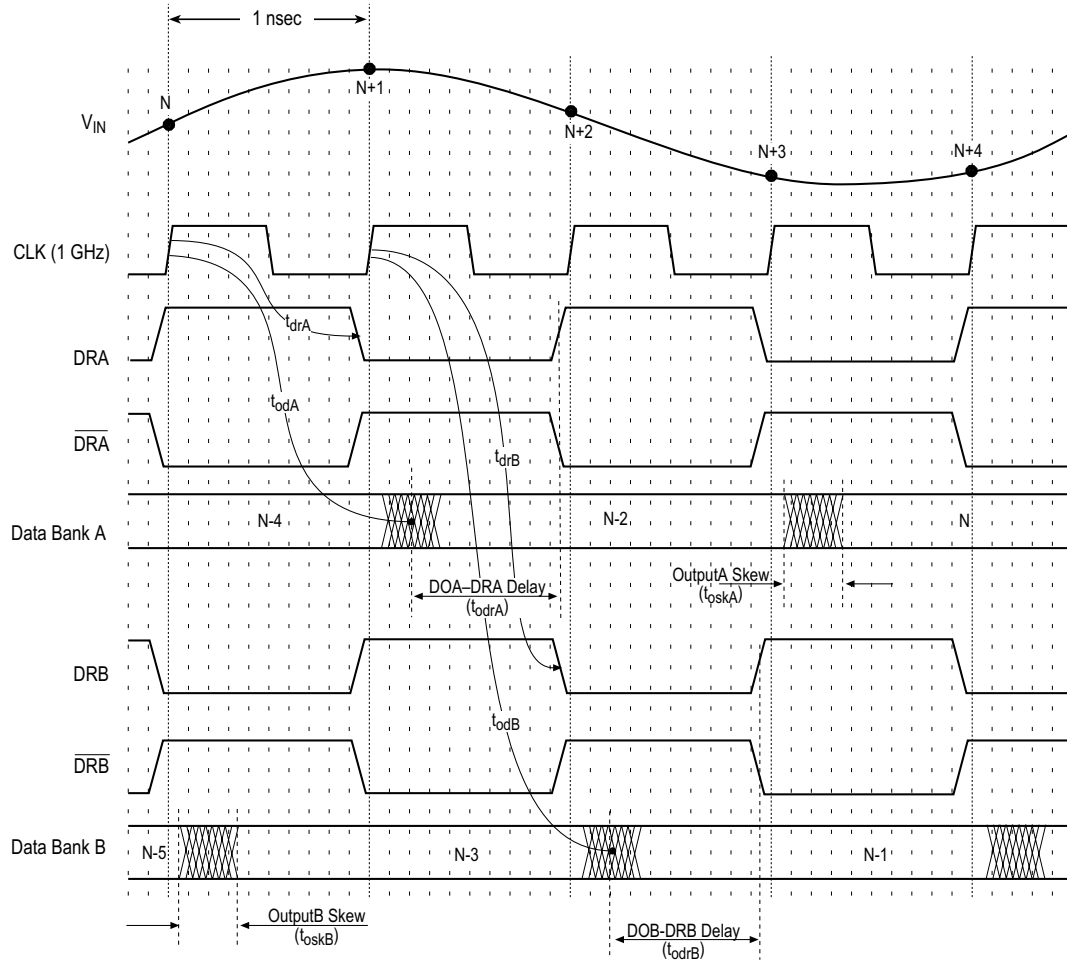
Figure 2 – Test Mode Timing Diagram
