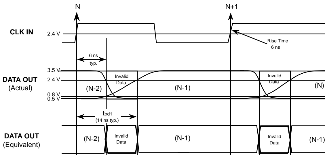
Figure 4 - Digital Output Characteristics
